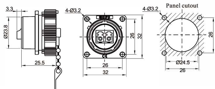
Square flange receptacle Mate with WY24JLCTE
