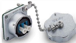
Square flange receptacle Mate with WY24JLCTE
