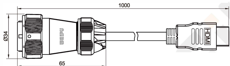
Plug with metal clamping-nut Mate with WY24KHDMI2.0Z
