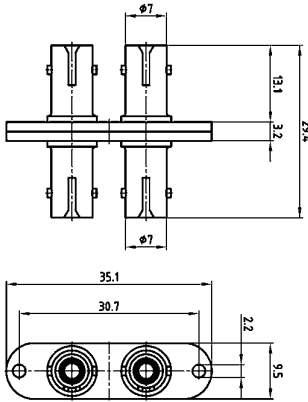
Duplex-Adapter
