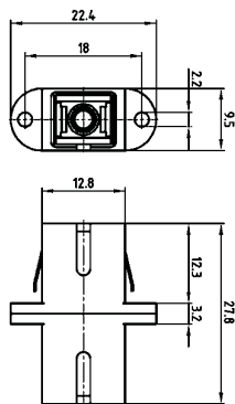
Simplex-Adapter
