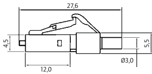
Connector
