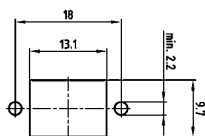
Panel cutout
