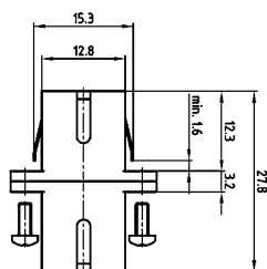
Simplex-Adapter
