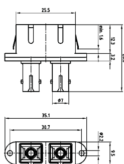
Duplex-Adapter plastic
