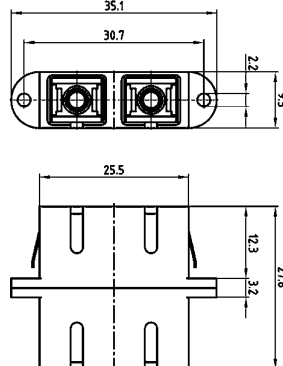
Duplex-Adapter
