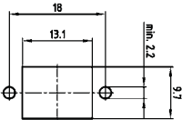
Panel cutout
