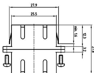
Duplex-Adapter
