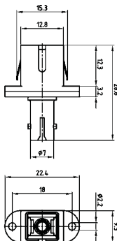
Simplex-Adapter plastic
