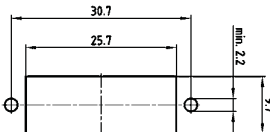
Panel cutout
