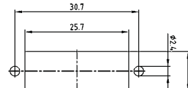
Panel cutout
