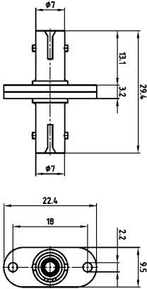
Simplex-Adapter
