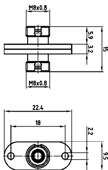
Simplex-Adapter plastic
