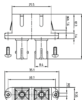
Duplex-Adapter metal
