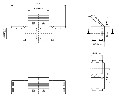
Duplex clip
