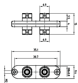
Duplex-Adapter metal
