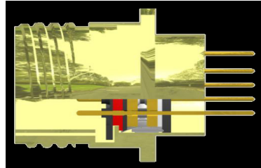
Mil-Spec Footprints: X2Y, Varistor Array, or Capacitive Planar Filter
